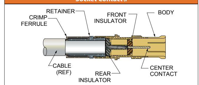
Socket Contact
