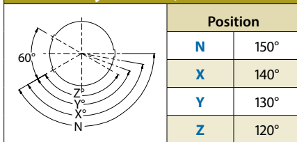
Master Key Positions, Shell Size 7-12
