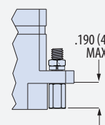
P Female Jackpost with Hex Nut and Lockwasher
