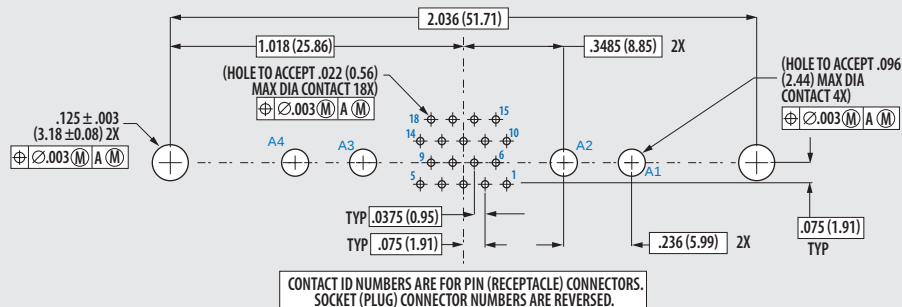
Contact numbers are mating face of pin connector. Socket connector contact numbers are reversed.
