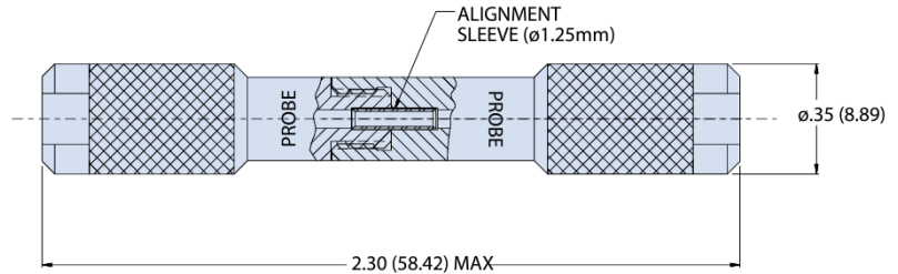
Probe-to-Probe Adapter
