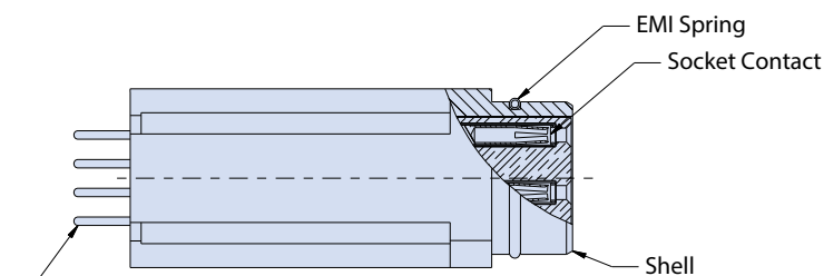
PC Tail Contacts
