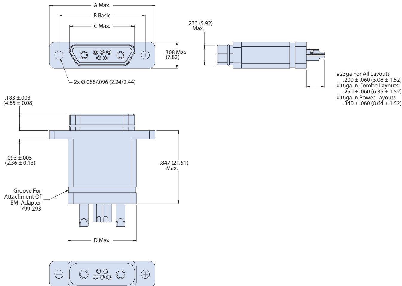
Shell Sizes A,B,C,D,E,F,J,K
