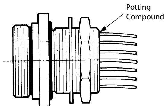
BULKHEAD RECEPTACLE WITH PIGTAILS
