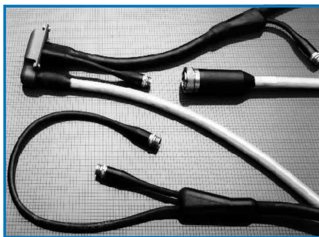
BULKHEAD RECEPTACLE WITH PIGTAILS
