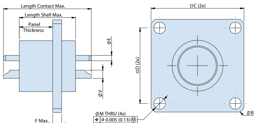
00 - Front Panel Mount Square Flange Receptacle with Accessory Mounting Threads
