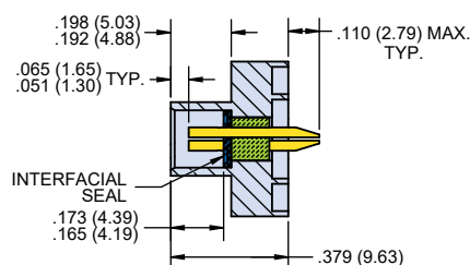
SOLDER CUP CONTACTS
