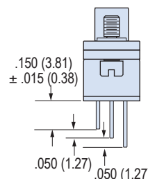
STAGGERED LEADS
