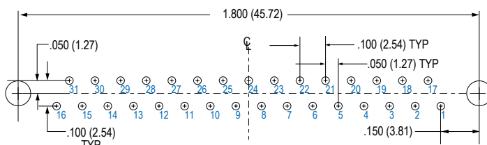
31 PIN
