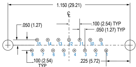
15 PIN
