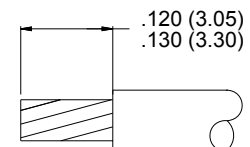
RECOMMENDED WIRE STRIP LENGTH
