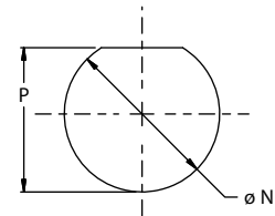
-07 PANEL CUT-OUT
