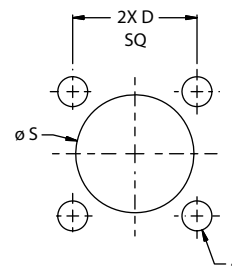
-02 PANEL CUT-OUT
