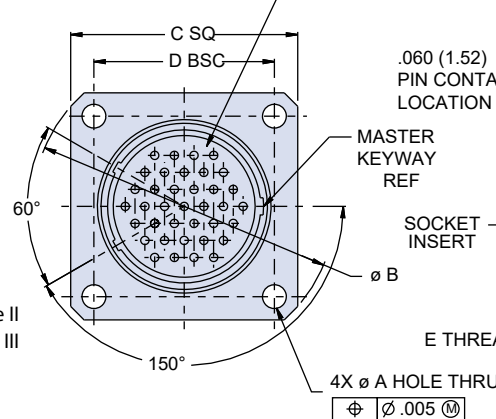
Square Flange Mount Dimensions
