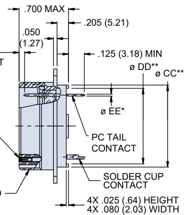
Square Flange Mount Dimensions
