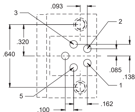
ARRANGEMENT NO. 10-5 (5 #16 CONTACTS)
