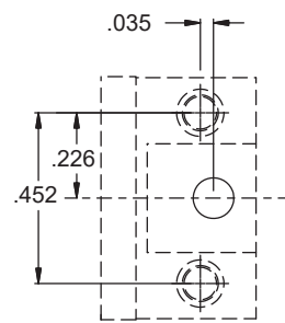
ARRANGEMENT NO. 7-1 (1 #12 CONTACT)
