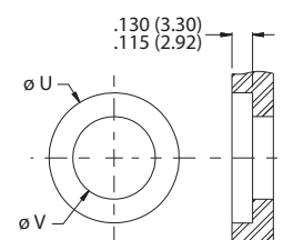
RECOMMENDED PANEL CUTOUT SHELL STYLE -13
