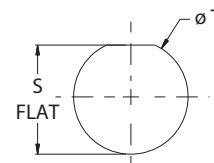
RECOMMENDED PANEL CUTOUT SHELL STYLE -07
