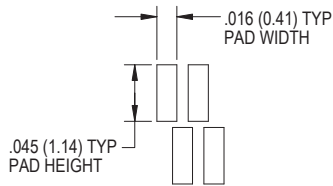
PAD FOOTPRINT DETAIL
