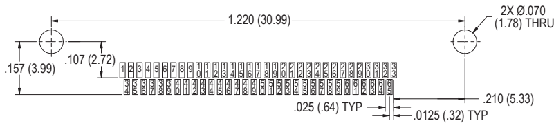
PAD FOOTPRINT DETAIL
