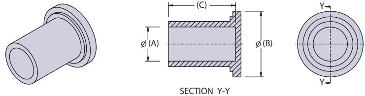
899-023 Circular Dust Covers
