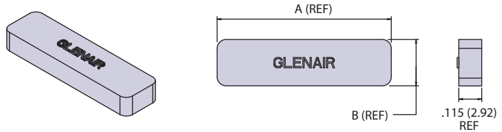
899-018 Rectangular Front Panel Mount Dust Covers
