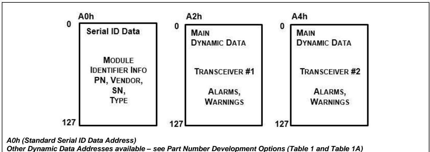
FIGURE 4 – DIGITAL DIAGNOSTIC MEMORY MAP OVERVIEW
