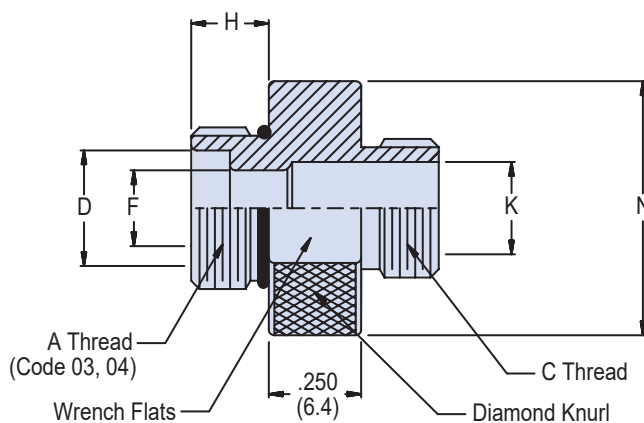
Style 02 Adapter with Internal Class 2B Thread (Code 03 and 04)
