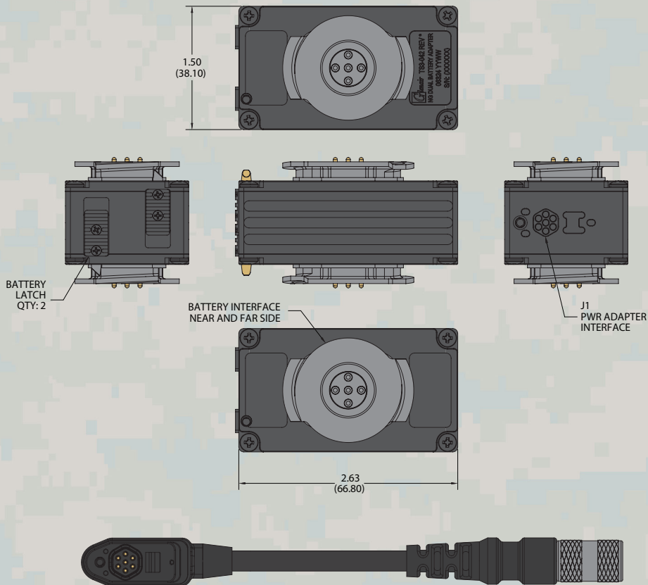
TS1-112 POWER ADAPTER CABLE INCLUDED
