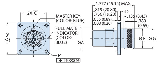
HS / HM - WALL MOUNT RECEPTACLE WITH HELICOILS
