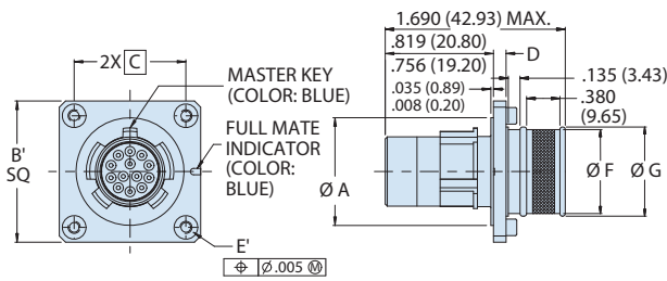
CS / CM - WALL MOUNT RECEPTACLE WITH CLINCH NUTS
