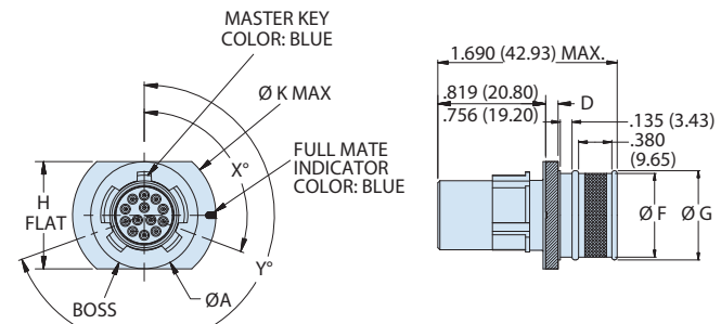
05 - IN-LINE RECEPTACLE
