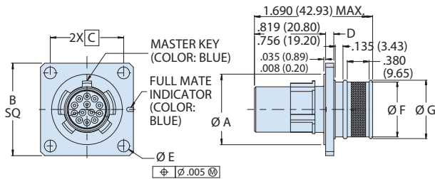
D0 - WALL MOUNT RECEPTACLE WITH ROUND HOLES
