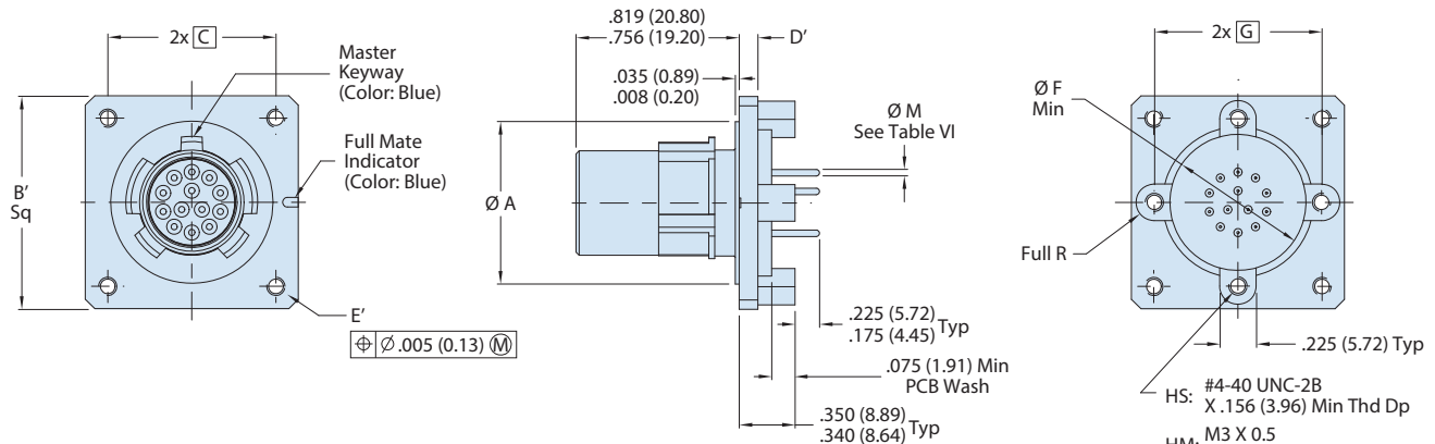
HS/ HM- WALL MOUNT RECEPTACLE WITH HELICOILS
