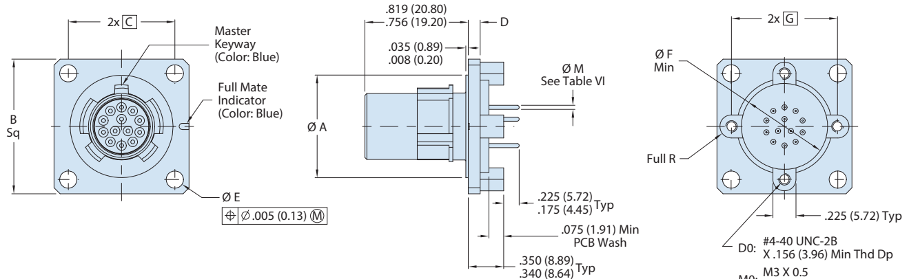
D0 / M0 - WALL MOUNT RECEPTACLE WITH ROUND HOLES
