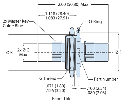
JAM NUT RECEPTACLE 234-105-44 (REF: MIL-DTL-38999/44)
