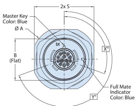
JAM NUT RECEPTACLE 234-105-44 (REF: MIL-DTL-38999/44)
