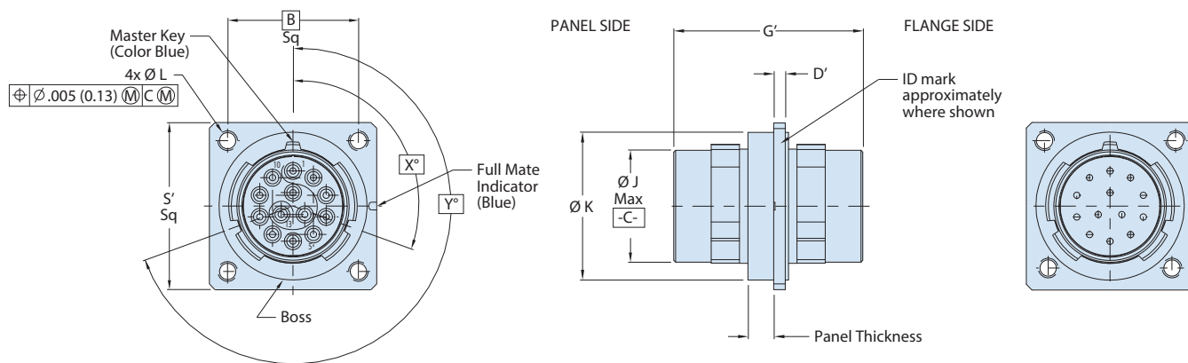
HS - WALL MOUNT RECEPTACLE STANDARD HELICOIL (SEE TABLE V)
