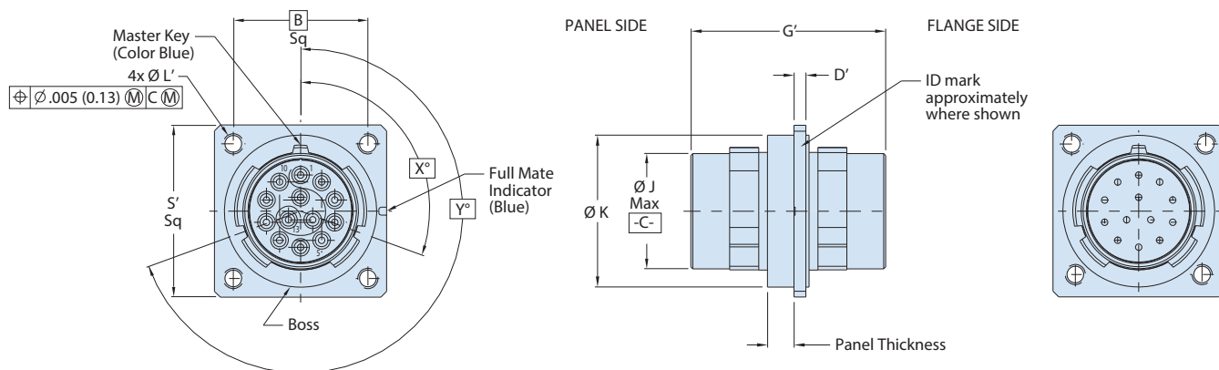
HM - WALL MOUNT RECEPTACLE METRIC HELICOIL (SEE TABLE V)
