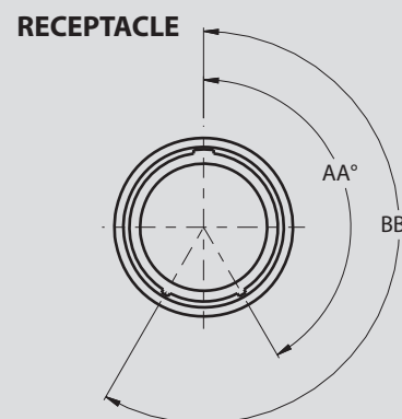
Normal and Alternate Position Keyway Rotation (Receptacle)
