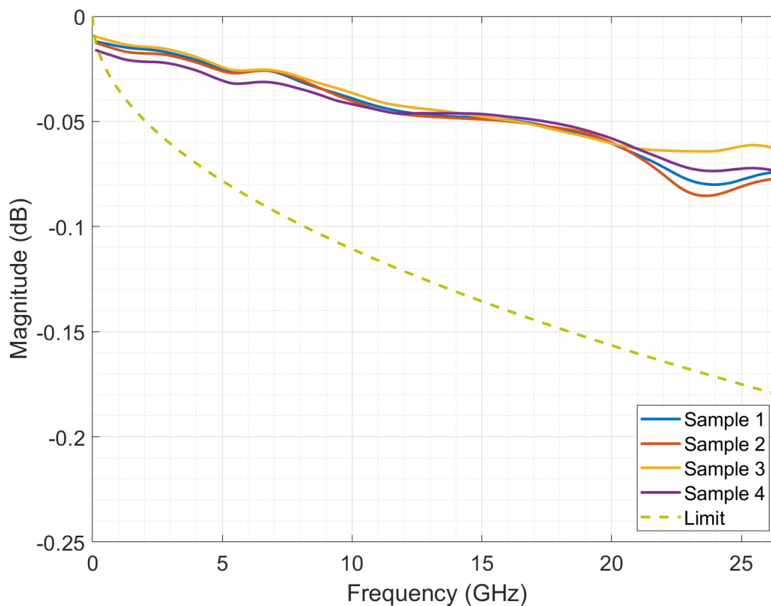
Figure 2. Connector Insertion Loss
