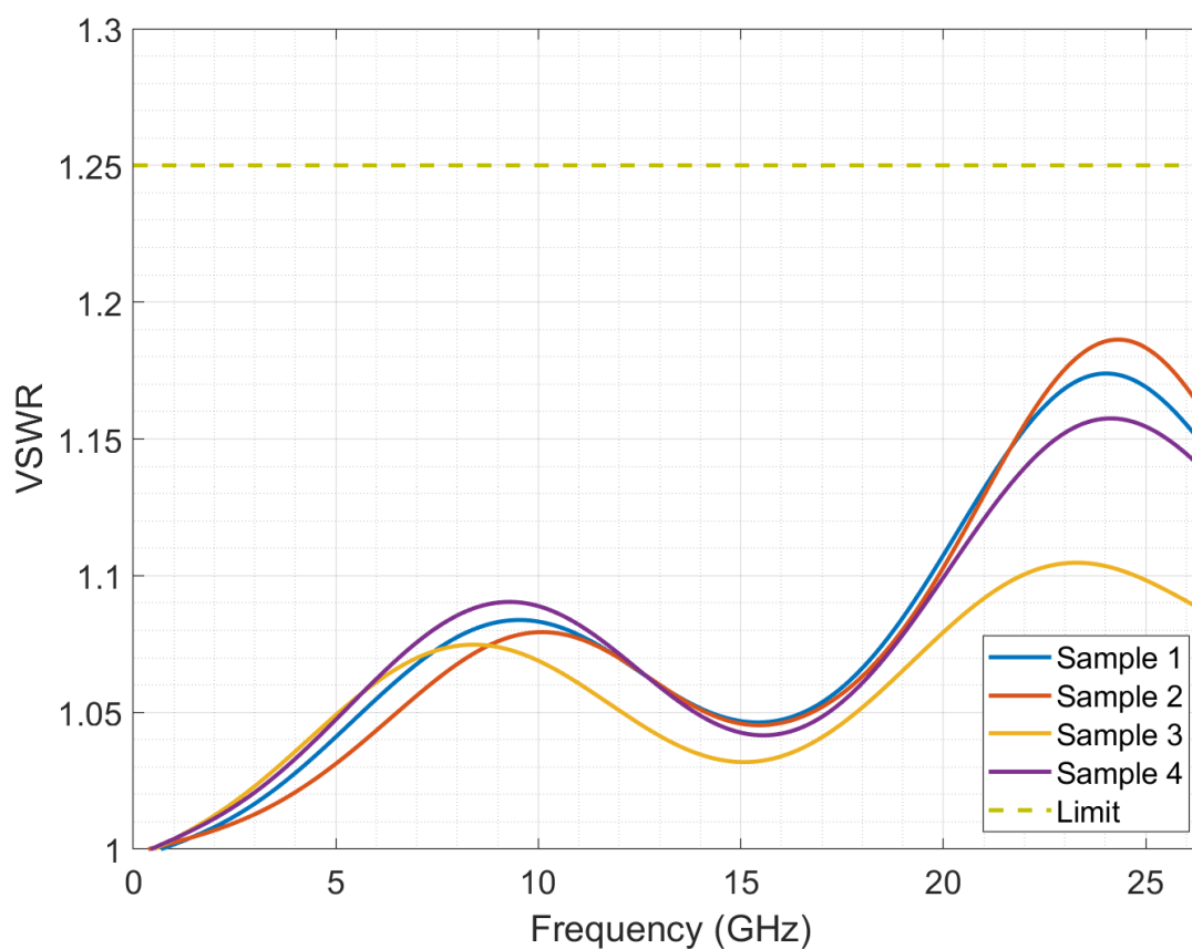
Figure 3. Connector VSWR
