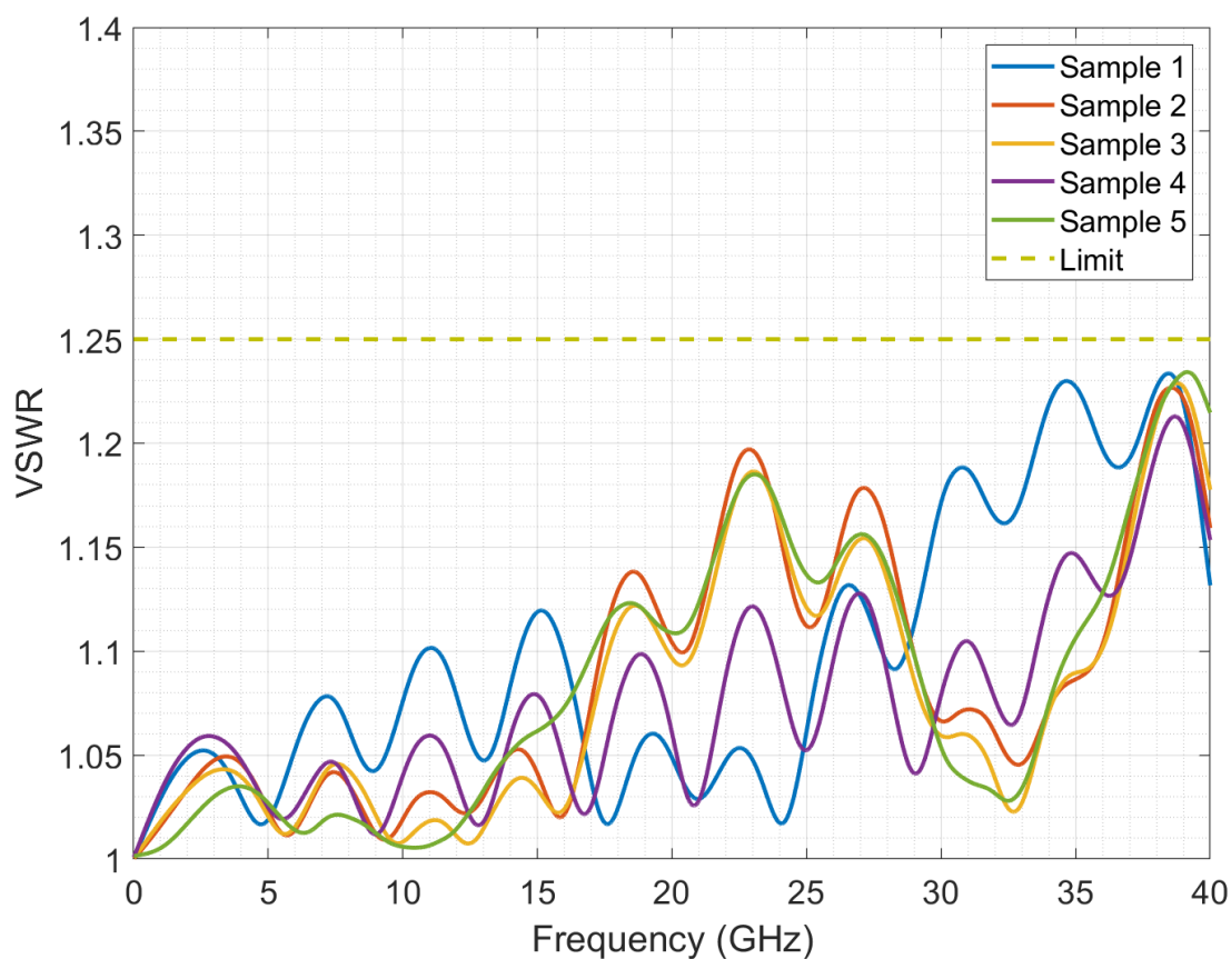
Figure 3. Connector VSWR
