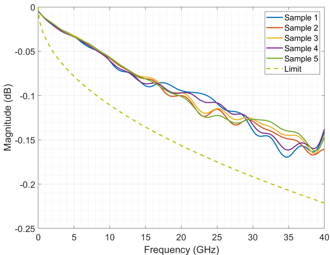
Figure 2. Connector Insertion Loss
