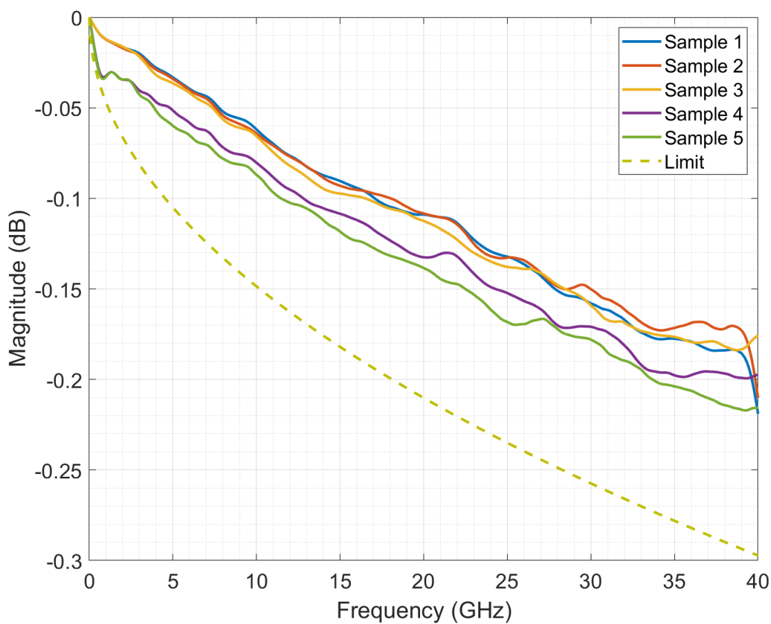
Figure 2. Connector Insertion Loss
