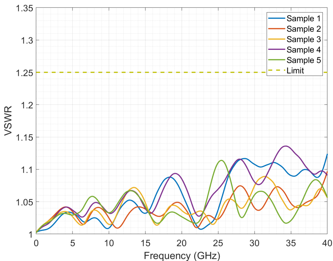
Figure 3. Connector VSWR
