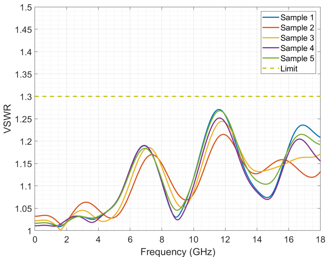
Figure 3. Connector VSWR
