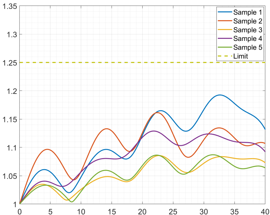
Figure 3. Connector VSWR
