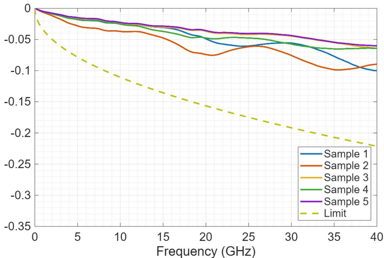
Figure 2. Connector Insertion Loss
