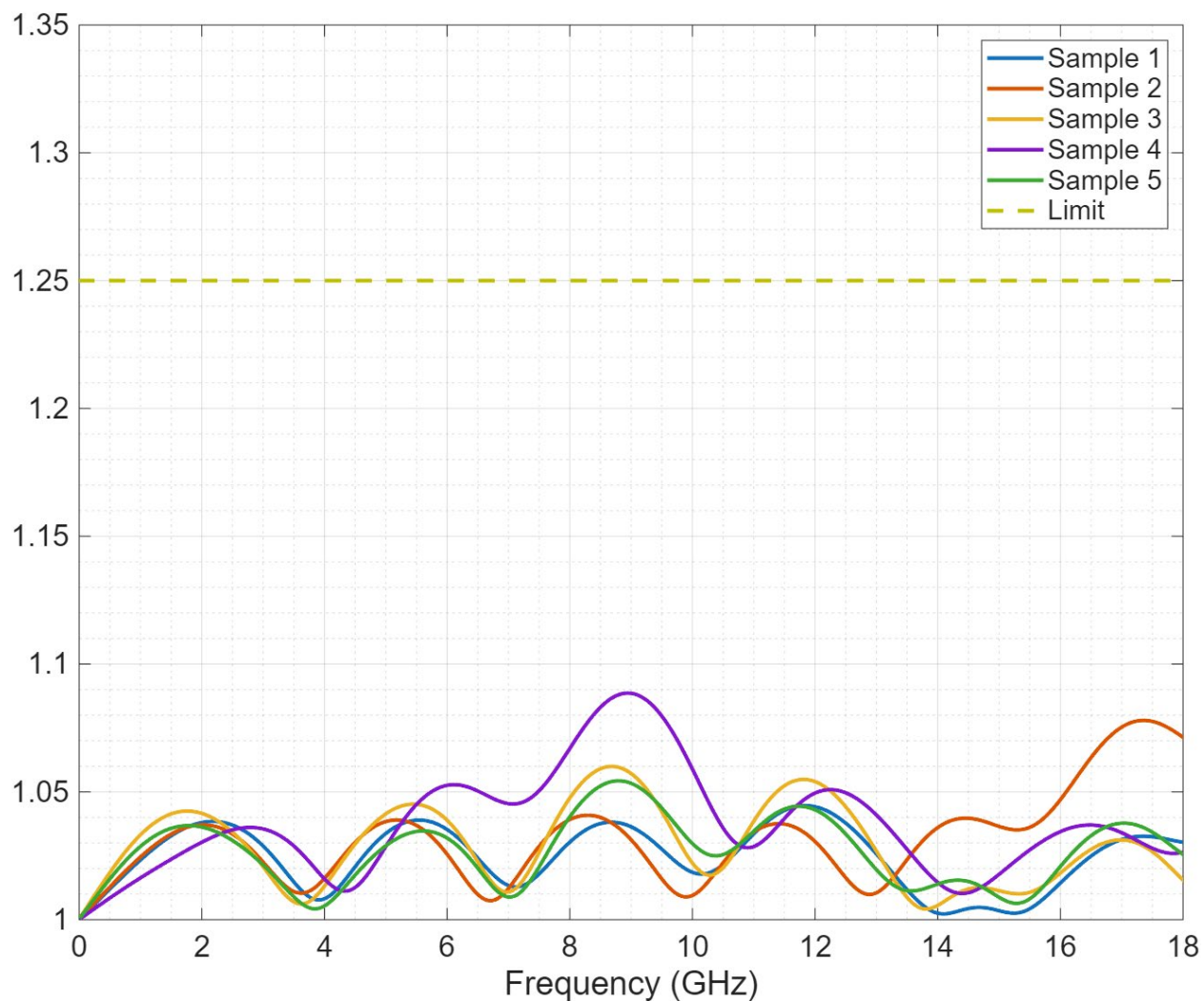
Figure 3. Connector VSWR
