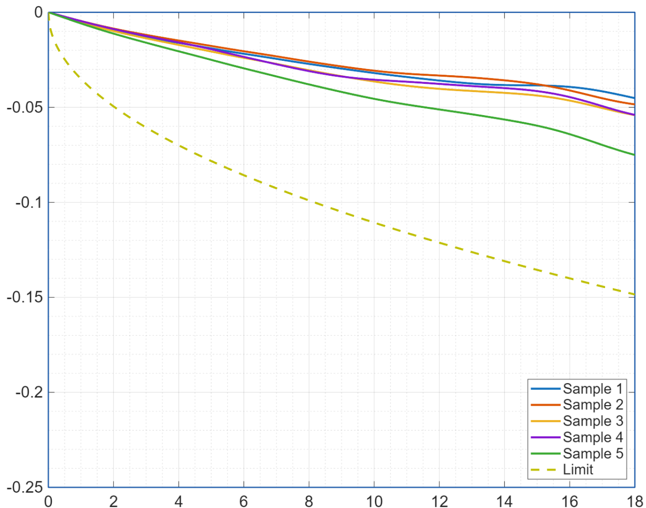
Figure 2. Connector Insertion Loss
