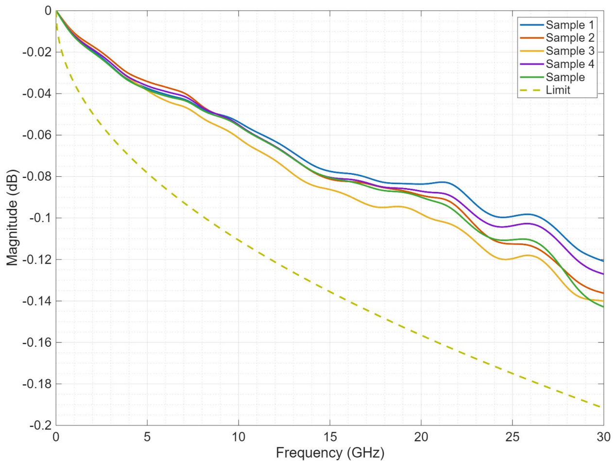
Figure 2. Connector Insertion Loss
