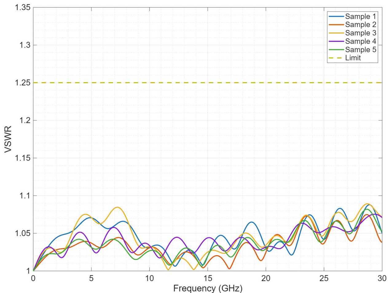
Figure 3. Connector VSWR
