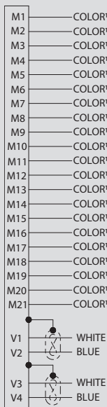
2-21 POSITION SIZE 37
