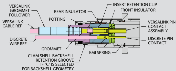
794-006 FLOAT-MOUNT RECEPTACLE
