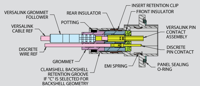
794-004 REAR PANEL-MOUNT RECEPTACLE
