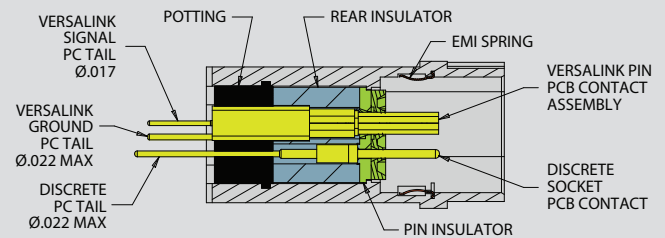
794-008 PCB-MOUNT RECEPTACLE
