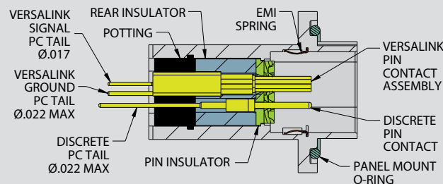
794-010 PCB-MOUNT RECEPTACLE
