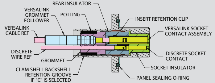
794-003 REAR PANEL-MOUNT PLUG
