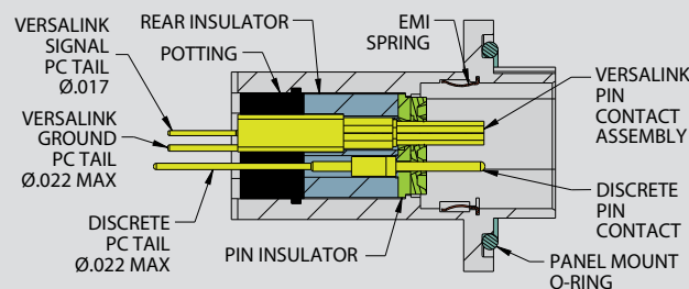
794-010 PCB-MOUNT RECEPTACLE
