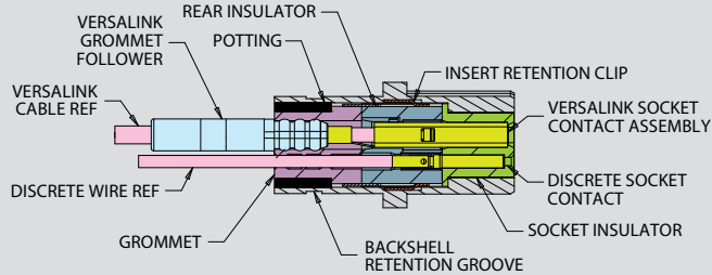
794-001 CABLE PLUG
