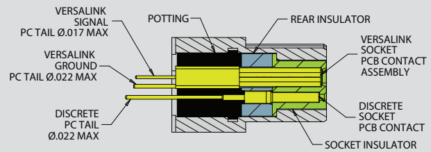
794-007 PCB-MOUNT PLUG
