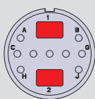
Insert Arrangement Mating Face View of Pin Contacts
