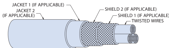
CABLE CONSTRUCTION EXAMPLE
